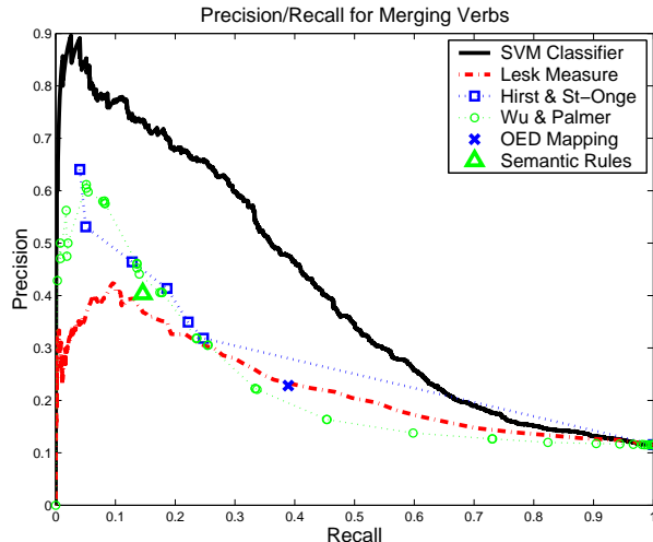
Figure 4: Precision/Recall plot for verb sense merge judgments
