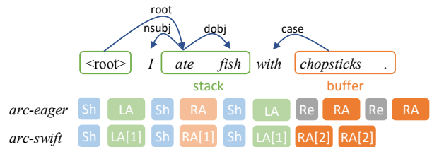
Figure 1: An example of the state of a transition-based dependency parser, and the transition sequences used by arc-eager and arc-swift to induce the correct parse. The state shown is generated by the first six transitions of both systems.
