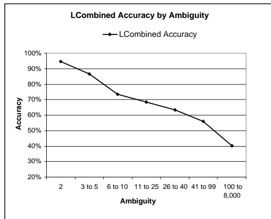
Figure 4. Parse ranking accuracy of LCombined by number of possible parses.
