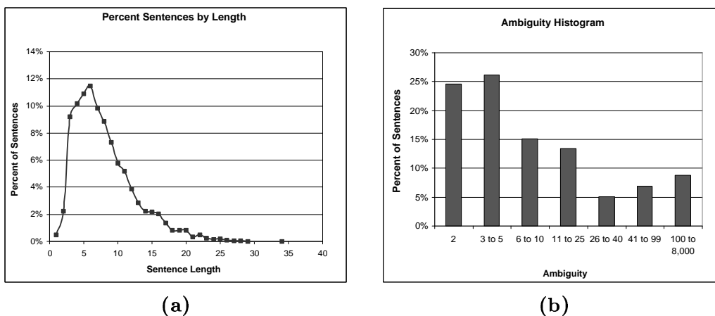
Figure 3. Percentage of sentences by length (a) and percentage of sentences by ambiguity level ranges (b) for the 3 rd Growth of the Redwoods corpus.
