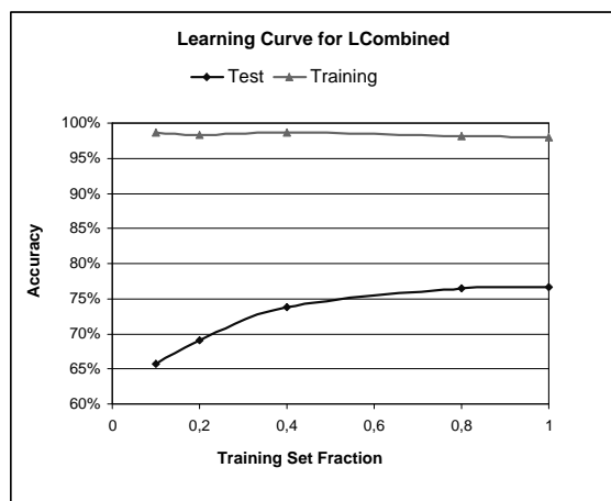
Figure 5. Learning curve for the model LCombined.
