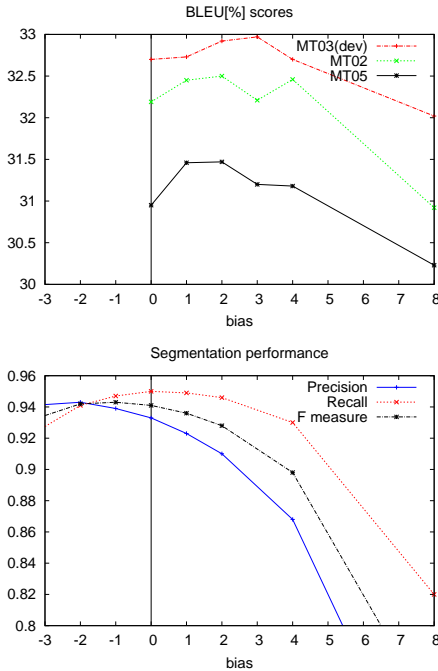
Figure 1: A bias towards more segment boundaries ( \lambda_0 > 0 ) yields better MT performance and worse segmentation results.
