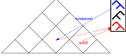
Figure 4: A schematic illustration of a parsing action, specified by a derivation on the agenda. First, we remove it from the agenda and put it in the chart. Then, combine it with other chart derivations to produce new derivations, which are added back to the agenda.
