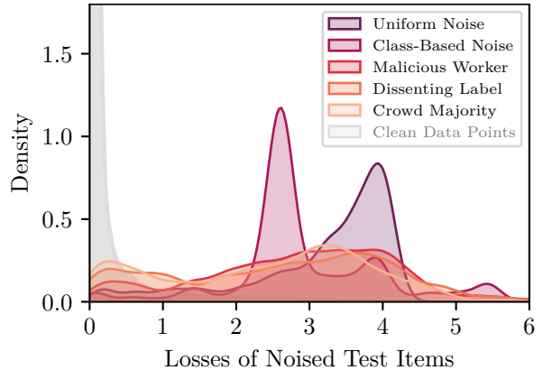
Figure 8: Distributions of losses of label errors on SNLI at 5% noising, which demonstrates similar performance characteristics to TweetNLP, as shown in Fig. 4.
