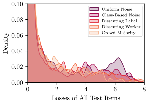
Figure 9: Combined distributions of losses of both noisy and clean data points, for TweetNLP with 5% noising.
