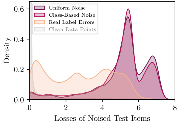
Figure 5: Distributions of losses of hypothesized label errors that MTurk workers verified for IMDB. As with Fig. 4, uniform and class-based methods do not approximate real, worker-identified errors, and losses of real label errors have greater overlap with the distribution of clean data; §6.
