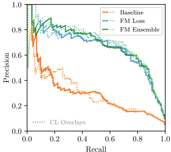
Figure 1: Precision-recall curves for label error detection: Large language models detect label errors with high precision, and far more effectively than a baseline word vector-based neural classifier. Overlaying a state-of-the-art model-agnostic error detection method, Confident Learning, results in little to no improvement (TweetNLP-5; §7).
