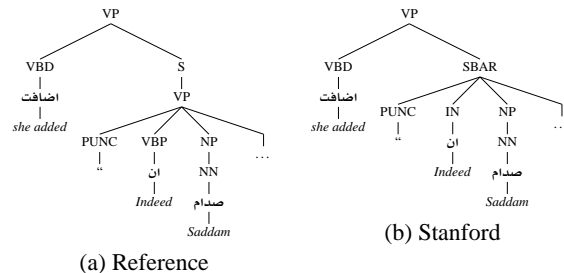
Figure 1: The Stanford parser (Klein and Manning, 2002) is unable to recover the verbal reading of the unvocalized surface form ان an (Table 1).
