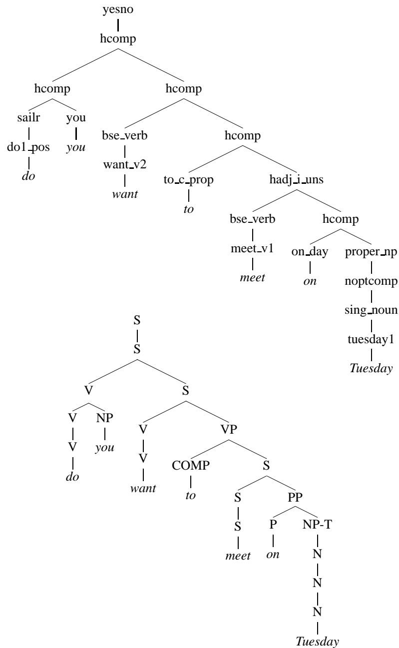
Figure 2: Native and derived Redwoods representations for the sentence Do you want to meet on Tuesday? (taken from the current development corpus): (a) derivation tree using unique rule and lexical item identifiers of the source grammar (top) and (b) phrase structure tree labelled with user-defined, parameterizable category abbreviations (bottom)
