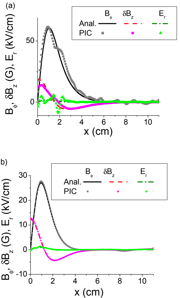
Figure 1: Comparison of analytical theory and particle-in-cell simulation results for the self-magnetic field; perturbation in the solenoidal magnetic field; and the radial electric field in a perpendicular slice of the beam pulse. The beam parameters are (a) n_{b0} = n_p/2 = 1.2 \times 10^{11} \text{cm}^{-3} , and (b) n_{b0} = n_p/8 = 0.6 \times 10^{11} \text{cm}^{-3} . The values of the applied solenoidal magnetic field, B_{z0} are: (a) B_{z0} = 300\text{G} ; and (b) B_{z0} = 600\text{G} .
