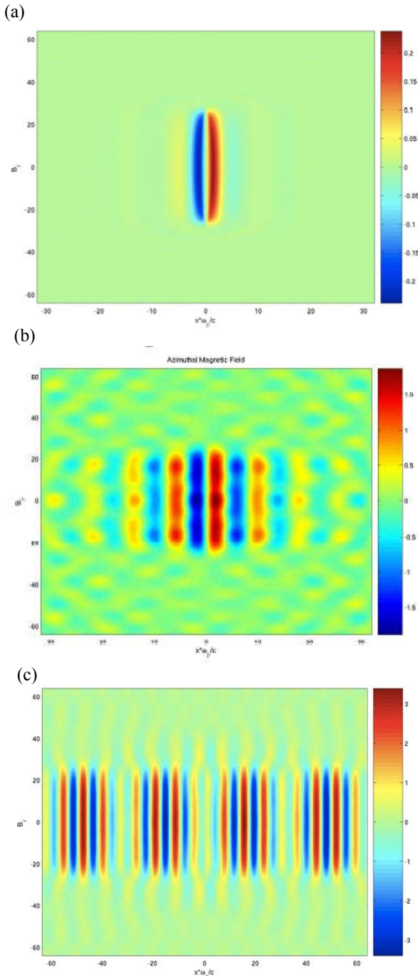
Figure 2: The two-dimensional profile of the self-magnetic field ( eB_y/2mc\omega_{pe} ) calculated according to Eq.(3) for a beam pulse with a flat-top profile and r_b = c/\omega_{pe} , l_b=20c/\omega_{pe} , and \beta_b = 0.5 for different values of the applied solenoidal magnetic field corresponding to (a) \omega_{ce} = \omega_{pe} , (b) \omega_{ce} = 1.32\omega_{pe} , and (c) \omega_{ce} = 1.35\omega_{pe} .
