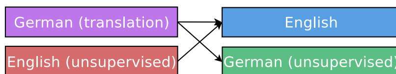
Figure 6.4: Many-to-many setting – multiple encoders, multiple decoders. I consider this scheme in a limited context of machine translation to utilize the large monolingual corpora in both the source and the target languages. Here, I consider a single translation task and two unsupervised autoencoder tasks.
