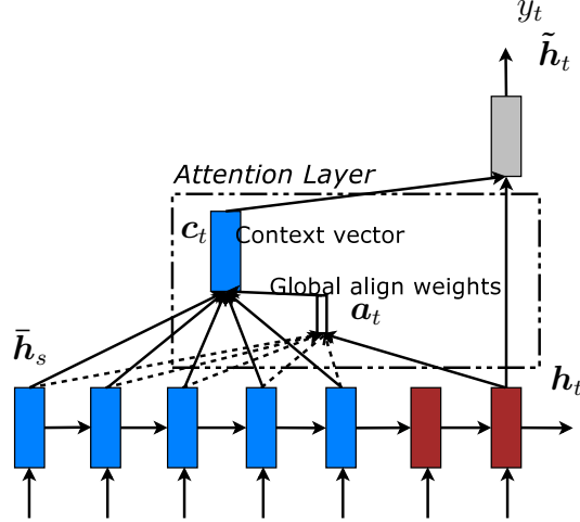
Figure 4.2: Global attentional model – at each time step t , the model infers a variable-length alignment weight vector \mathbf{a}_t based on the current target state h_t and all source states \bar{h}_s . A global context vector \mathbf{c}_t is then computed as the weighted average, according to \mathbf{a}_t , over all the source states.
