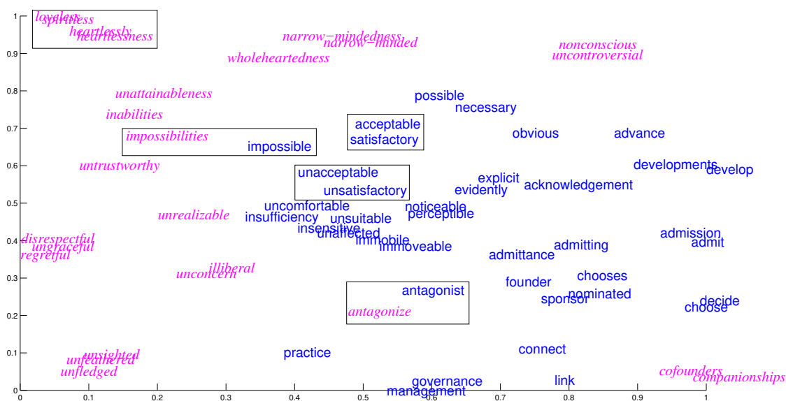
Figure 5.5: Barnes-Hut-SNE visualization of source word representations – shown are sample words from the Rare Word dataset. I differentiate two types of embeddings: frequent words in which encoder embeddings are looked up directly and rare words where I build representations from characters. Boxes highlight examples that I will discuss in the text. I use the hybrid model ( l ) in this visualization.
