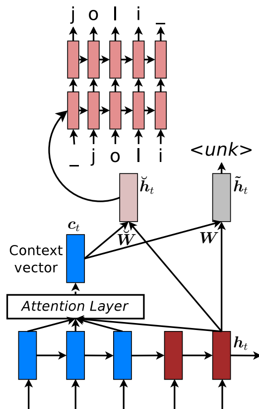
Figure 5.3: Separate-path target generation – two separate attentional vectors are creating: \tilde{h}_t for predicting target words and \check{h}_t to seed the target-side character model.
